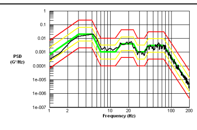
Block 12 Face 3 Test Vibration Profile
