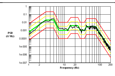
Block 12 Face 6 Test Vibration Profile
