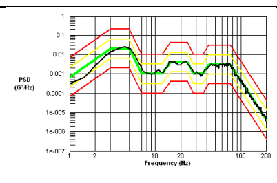
Block 12 Face 4 Test Vibration Profile
